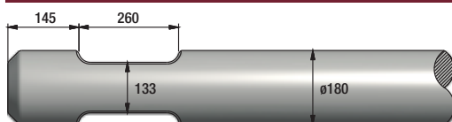
FIGURE 302 PROMOVE XP4500
