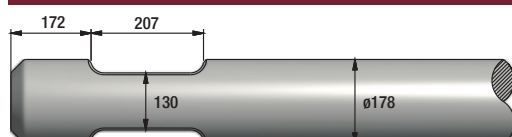
FIGURE 391 SOCOMEK MDO 4000
