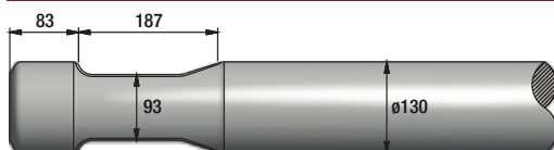
FIGURE 300 PROMOVE XP1500
