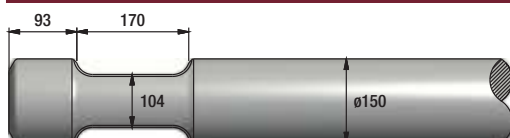
FIGURE 235 MSB SAGA 300
