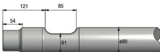
FIGURE 73 EVERDIGM EHB10
