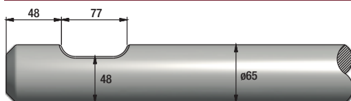
FIGURE 53 CATERPILLAR H65DS
