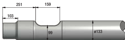
FIGURE 11 ARROWHEAD S230
