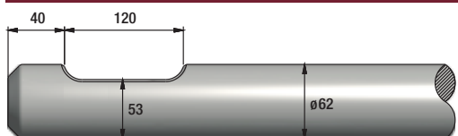
FIGURE 375 SOCOMEK DMS 210
