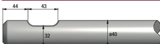
FIGURE 337 RAMMER BR255
