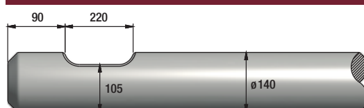
FIGURE 388 SOCOMEK MDO 1950
