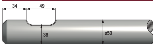
FIGURE 55 CATERPILLAR H45ES
