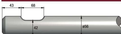
FIGURE 52 CATERPILLAR H55DS
