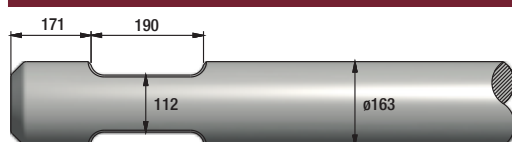
FIGURE 390 SOCOMEK MDO 3000 / 3200
