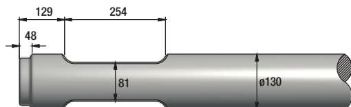
FIGURE 153 ITALDEM GK 1600
