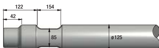
FIGURE 401 SOOSAN SB70 / 71
