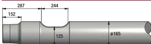
FIGURE 277 NPK E-225
