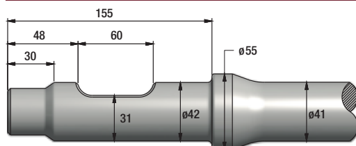
FIGURE 158 KRUPP HM45
