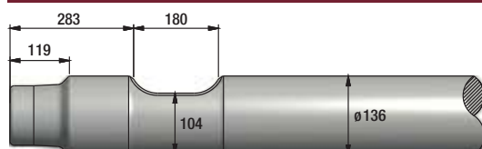
FIGURE 265 NPK GH10
