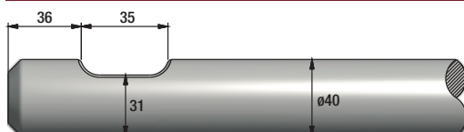
FIGURE 54 CATERPILLAR H35ES
