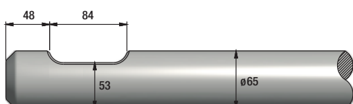
FIGURE 377 SOCOMEK DMS 270
