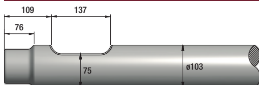
FIGURE 9 ARROWHEAD S130
