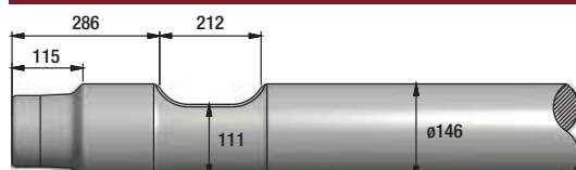
FIGURE 266 NPK GH12
