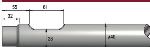
FIGURE 280 NPK H-06X
