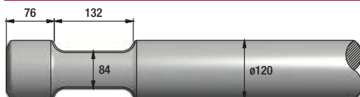
FIGURE 233 MSB SAGA 180
