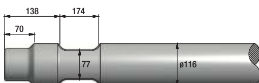
FIGURE 76 EVERDIGM EHB20
