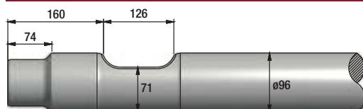
FIGURE 260 NPK E-206
