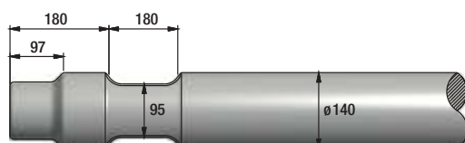
FIGURE 403 SOOSAN SB100
