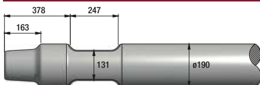
FIGURE 278 NPK E-235
