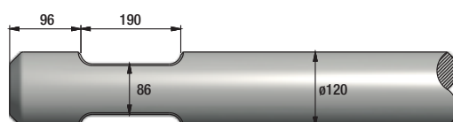
FIGURE 153 ITALDEM GK 1600
