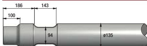
FIGURE 401 SOOSAN SB70 / 71
