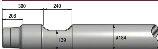
FIGURE 279 NPK E-240A
