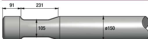
FIGURE 301 PROMOVE XP2400
