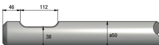
FIGURE 339 RAMMER BR333
