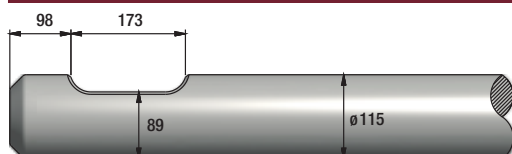
FIGURE 385 SOCOMEK MDO 750
