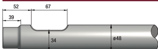
FIGURE 160 KRUPP HM60V
