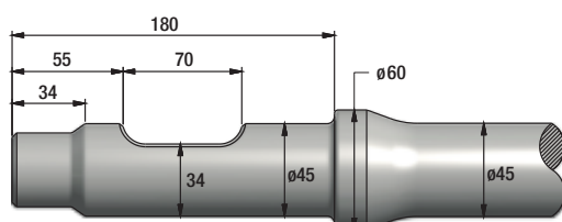
FIGURE 160 KRUPP HM60V
