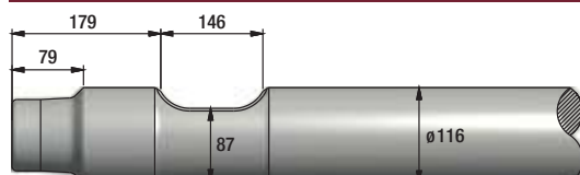
FIGURE 262 NPK E-208A
