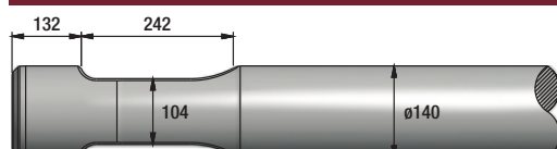
FIGURE 217 MONTABERT V1800
