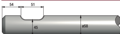
FIGURE 56 CATERPILLAR H55ES
