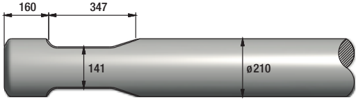
FIGURE 182 KRUPP HM4000
