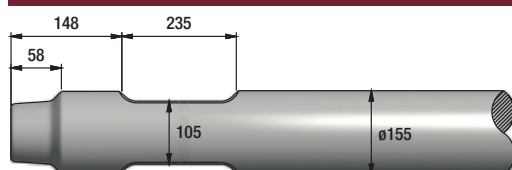
FIGURE 389 SOCOMEK MDO 2050
