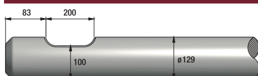
FIGURE 387 SOCOMEK MDO 1450
