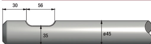
FIGURE 372 SOCOMEK DMS 50
