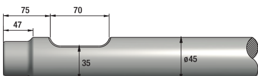
FIGURE 374 SOCOMEK DMS 160
