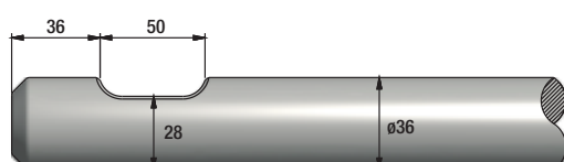
FIGURE 336 RAMMER BR222
