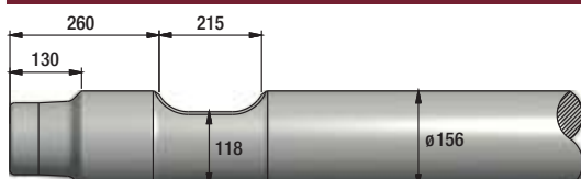
FIGURE 275 NPK E-220
