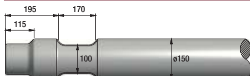
FIGURE 403 SOOSAN SB100
