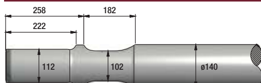
FIGURE 216 MONTABERT V1600
