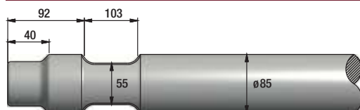
FIGURE 398 SOOSAN SB45
