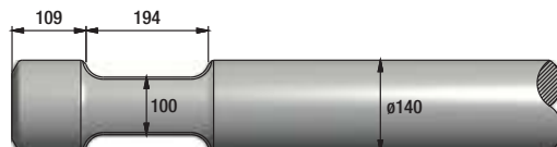
FIGURE 154 ITALDEM GK 1800
