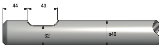
FIGURE 50 CATERPILLAR H35DS
