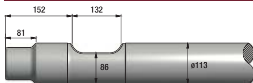
FIGURE 10 ARROWHEAD S180
